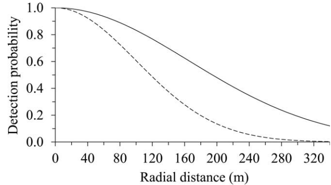
FIGURE 3. Detection probability of the Grenada Dove presented as a function of distance and time of day. Detection was modeled using the half-normal key function without series expansion and time of day as a continuous or factor covariate (solid line: 0630–0900, 1631–1900 hours; dashed line: 0901–1100, 1530–1630 hours).
